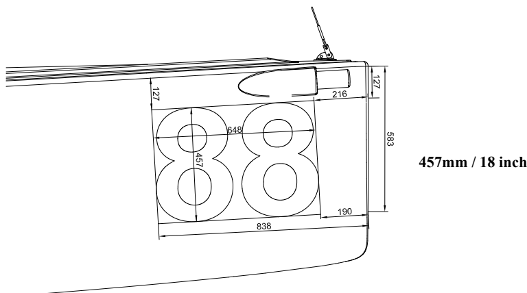
J/70 Class Bow Number Location & Size #2 Large number - height = 457mm (18") Dimensions in mm 6-11-2018
