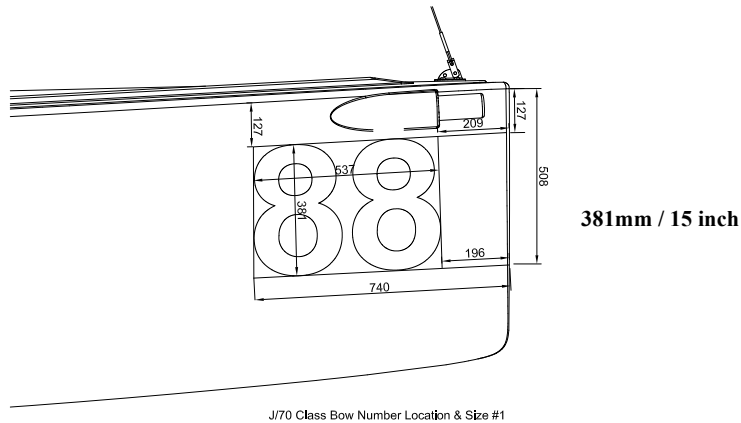
J/70 Class Bow Number Location & Size #1 Standard number - height = 381mm (15") Dimensions in mm 6-11-2018
